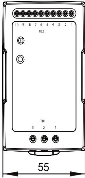
Terminal Pin No. Assignment (TB1)
