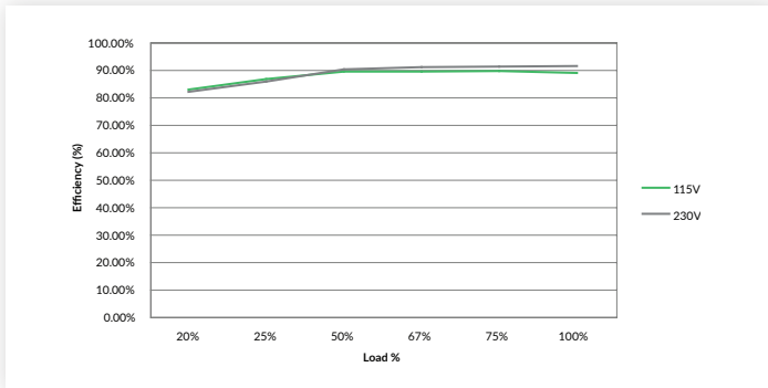
Figure 3 GCS250PS12
