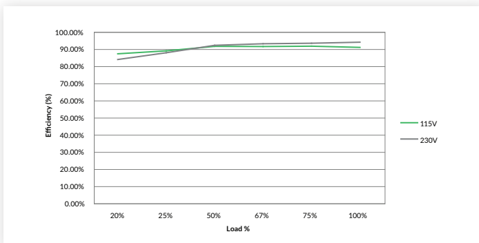
Figure 5 GCS250PS48
