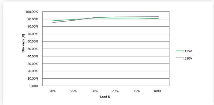
Figure 4 GCS250PS24
