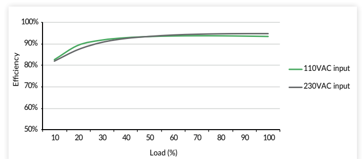
Figure 2 - UCH600PS24
