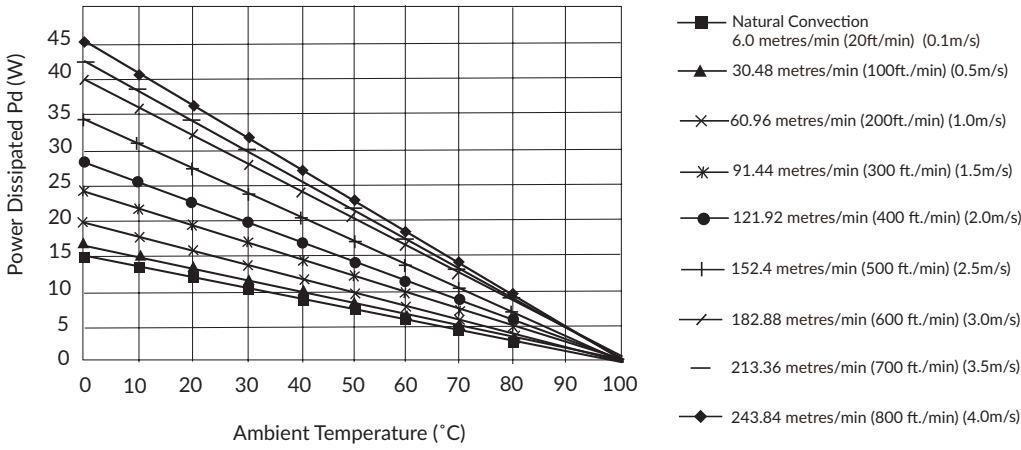
Forced Convection Power Derating without Heatsink
