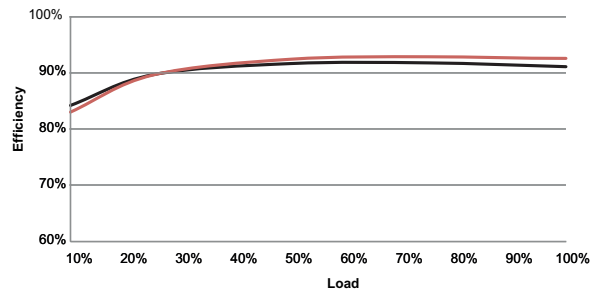
ALM120US12
