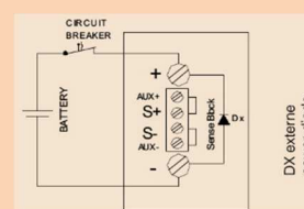
Remote Sensing (twisted sense lines)
